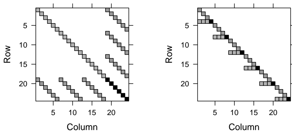
Figure 8: Structure of the sparse matrices \mathbf{A} (left panel) and \mathbf{L} (right panel) for the model Om1a.
