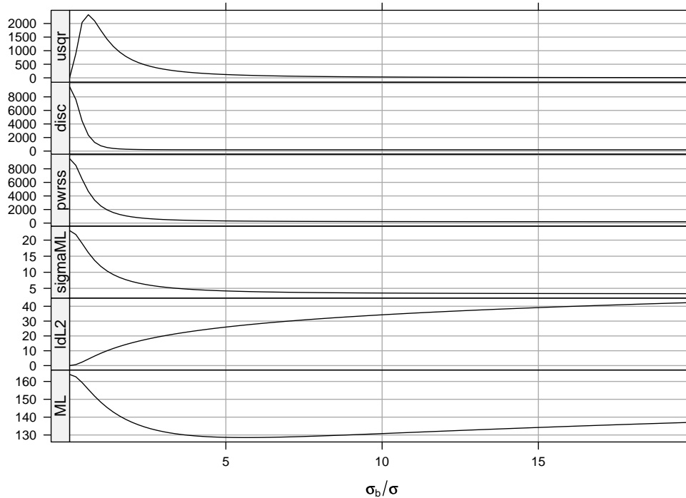
Figure 2: The profiled deviance, and those components of the profiled deviance that vary with \theta , as a function of \theta in model Rm1ML for the Rail data. In this model the parameter \theta is the scalar \sigma_1 , the standard deviation of the random effects relative to the standard deviation of the per-observation noise.
