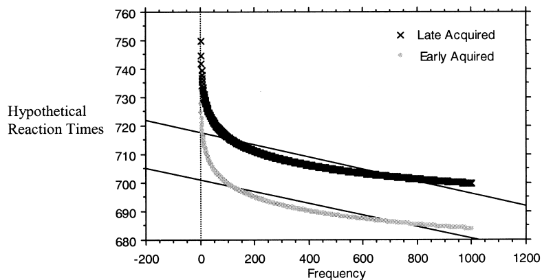
Fig. 1. Hypothetical data based on the revised cumulative-frequency hypothesis. Items vary in their frequency from 1 to 1000 and take values of being learnt 1 year ago (late-acquired) or 10 years ago (early-acquired). The reaction time for each item is calculated using Eq. (3) with A = 0.01 . The two simple regression lines show the linear correlation between reaction time and frequency for early- and late-acquired items. These lines are nearly parallel indicating that the two effects of frequency and AoA are additive.
