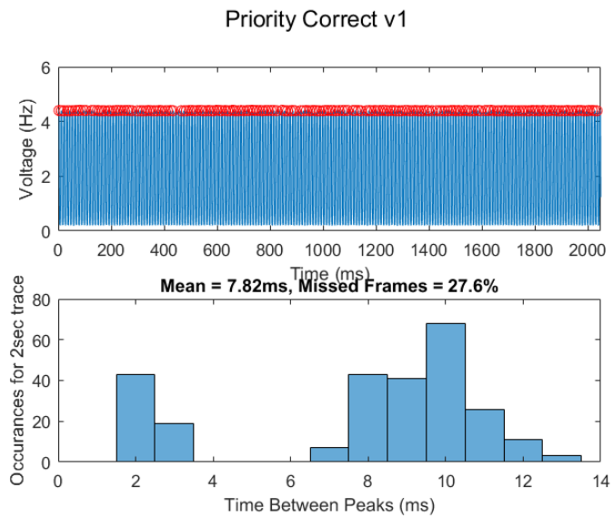
Figure 3: Correctly prioritizing experiment monitor
