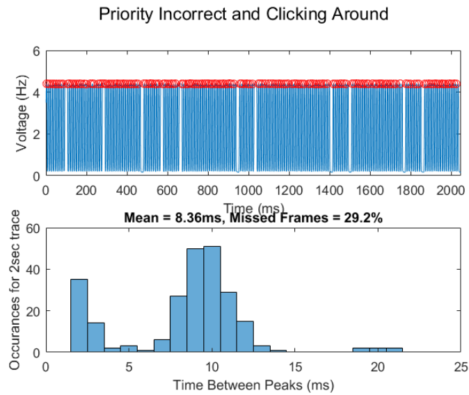
Figure 1: Clicking around on the experimenter monitor during experiment.
