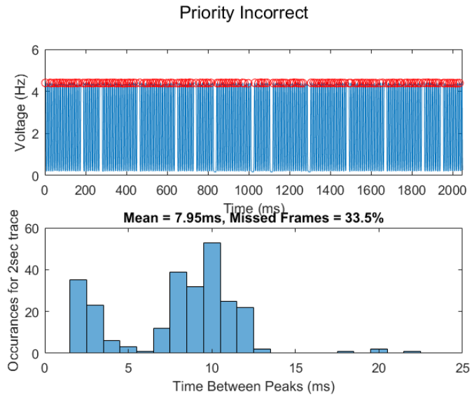
Figure 2: Not resetting the priority after clicking around.
