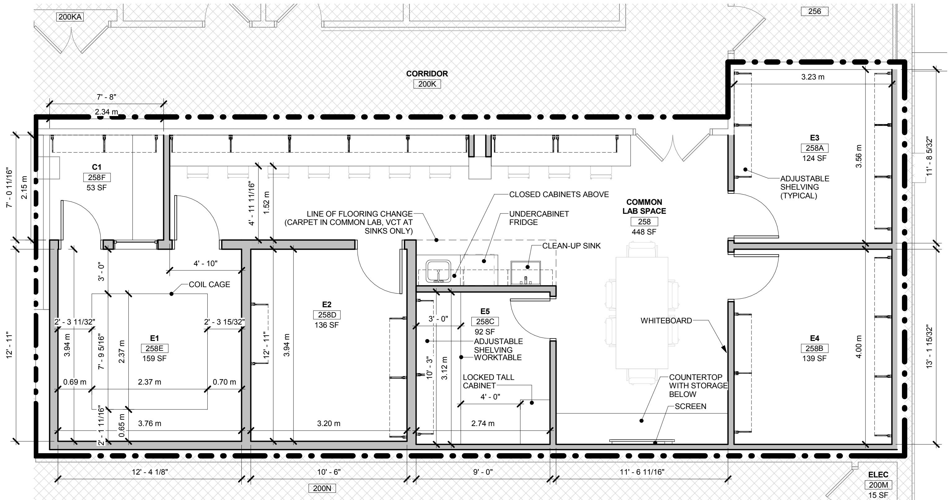
1 PROPOSED FLOOR PLAN- OPTION 2_REV 2 1/4" = 1'-0"
